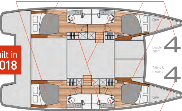
Fountaine Pajot Helia 44 - Sailing Catamaran
