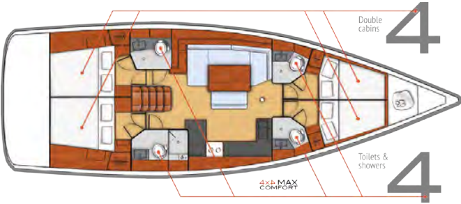
Beneteau Oceanis 48 - Sailing Yacht
