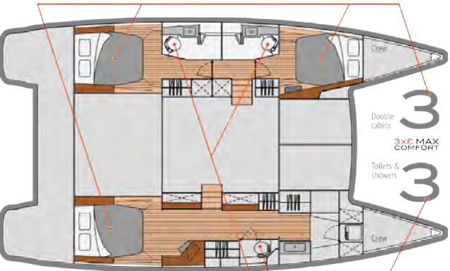
Fountaine Pajot Helia 44 - Sailing Catamaran
